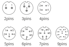
针位图 Male contact view
