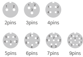
孔位图 Female contact view
